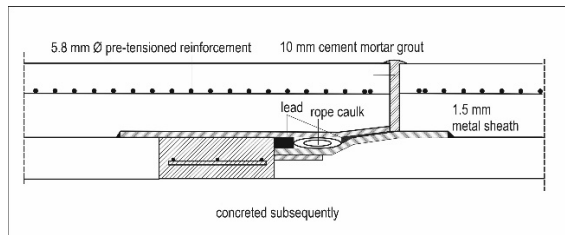
Diag. 3: Bonna-Rohr type (Steel casing/ sprayed concrete pipe) [DYWIDAG]
